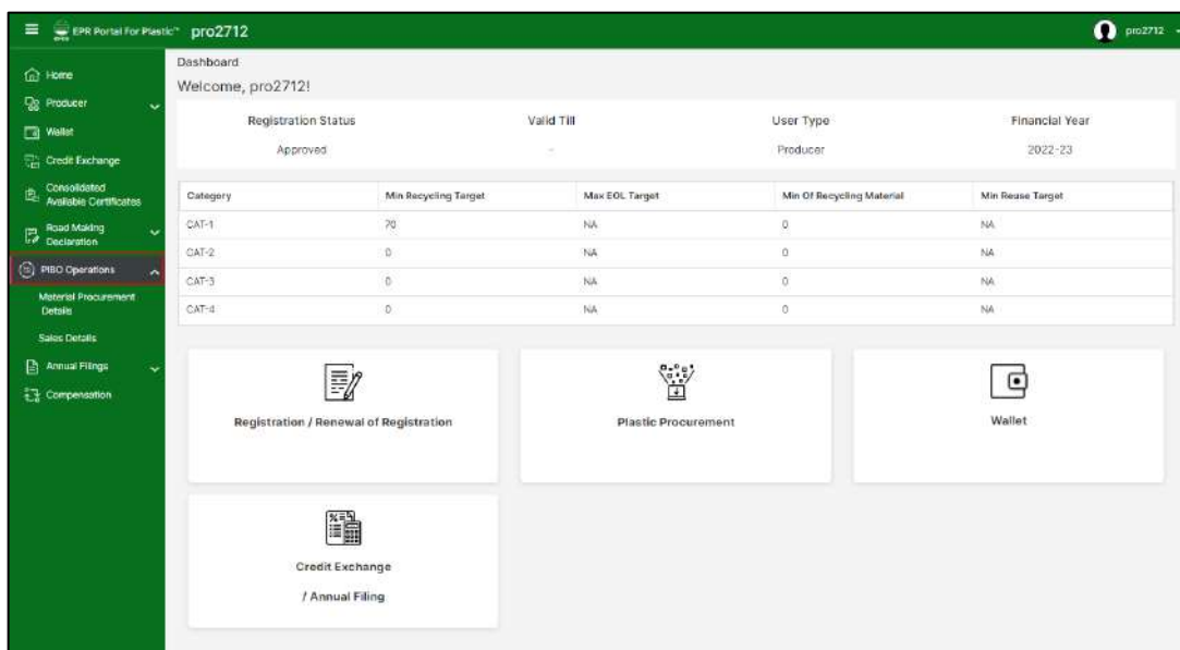
Figure 5.1: PIBOs Dashboard
